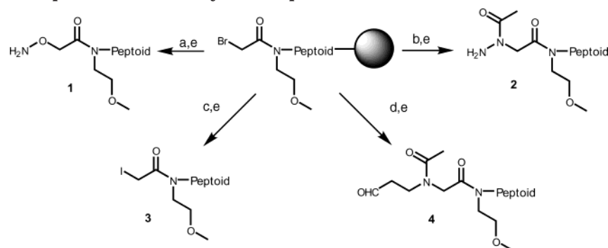
Scheme 1. Ligation Groups from Bromoacetylated Peptoids a
